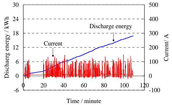
Fig. 8 Typical current and discharge energy curve during demonstration. Air conditioning was used
