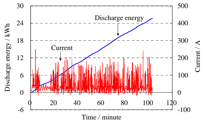
Fig. 9 Typical current and discharge energy curve during demonstration. Air conditioning was used
