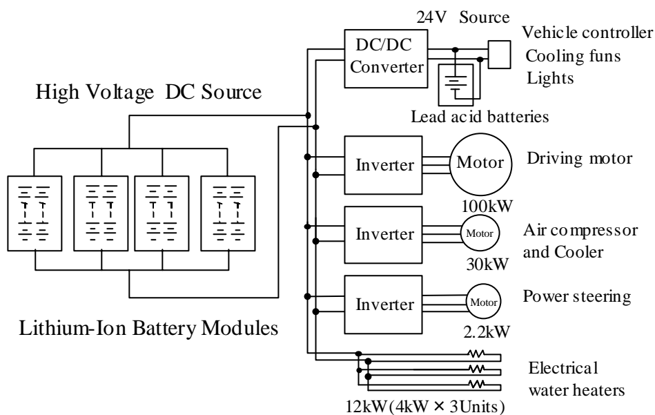
Fig.2 System configuration of the bus
