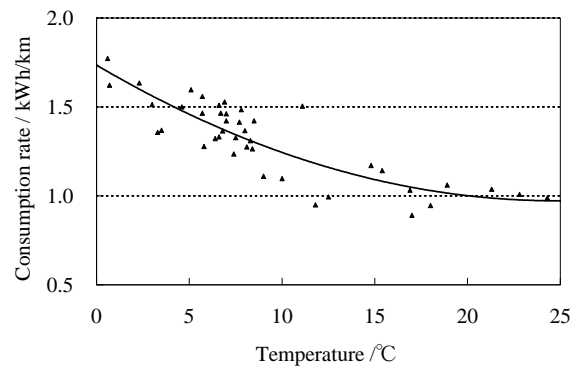
Fig.10 Relationship between temperature and energy consumption rate
