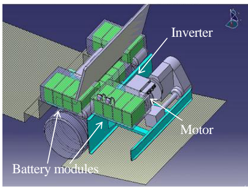
Fig.3 Battery modules, Motor, and Inverter installed in the bus
